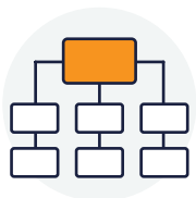
Smart Contract
